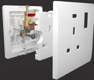
Socket Assembly
